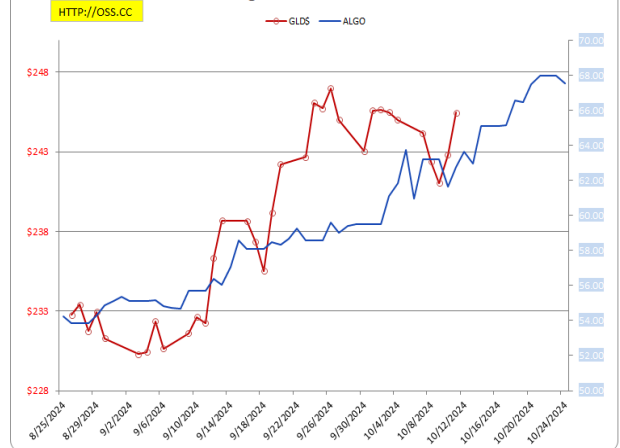
Algo Forecast vs GLD
